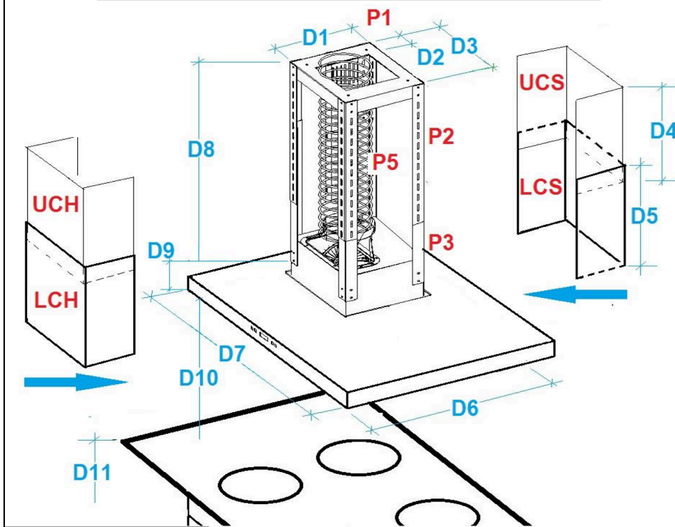
DIMENSION TABLE
